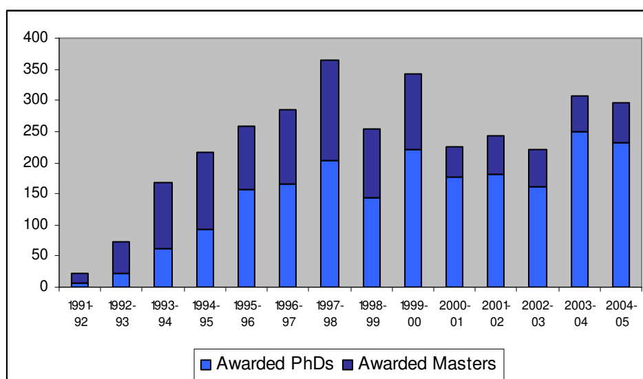
FIGURE 2.2: AWARDED DEGREES AT CRCs 1991-92 TO 2004-05
